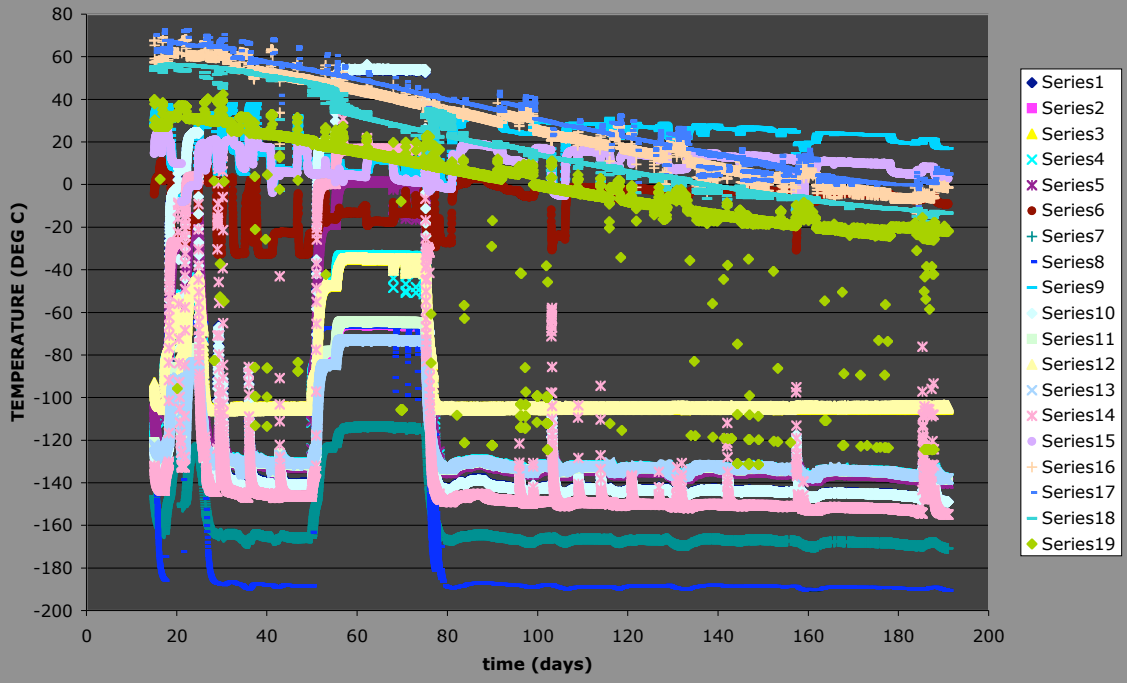
HRI Temperatures vs time
