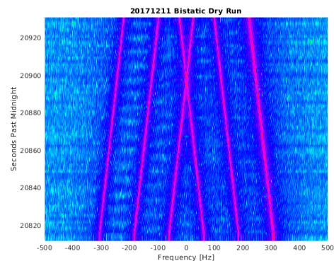
Figure 1. Data extracted from the KEM1 Cruise datasets for Solar conjunction (left) and Bistatic Dry Run (right), which match expectations based on the documentation (“rex_activities_kemcruise1.pdf”)
