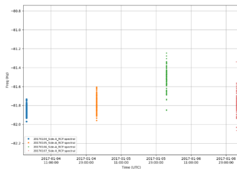
Figure 1. Data extracted from the KEM1 Cruise datasets for Solar conjunction (left) and Bistatic Dry Run (right), which match expectations based on the documentation (“rex_activities_kemcruise1.pdf”)
